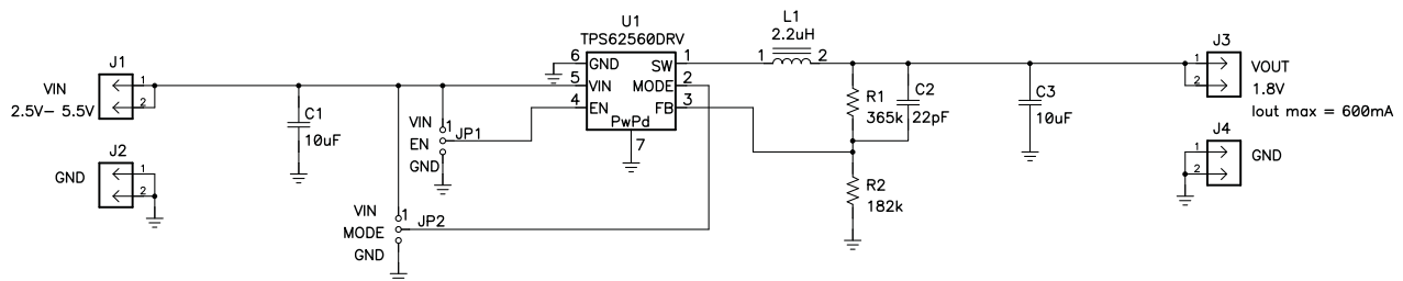
Figure 8. TPS62560EVM-330 Schematic
