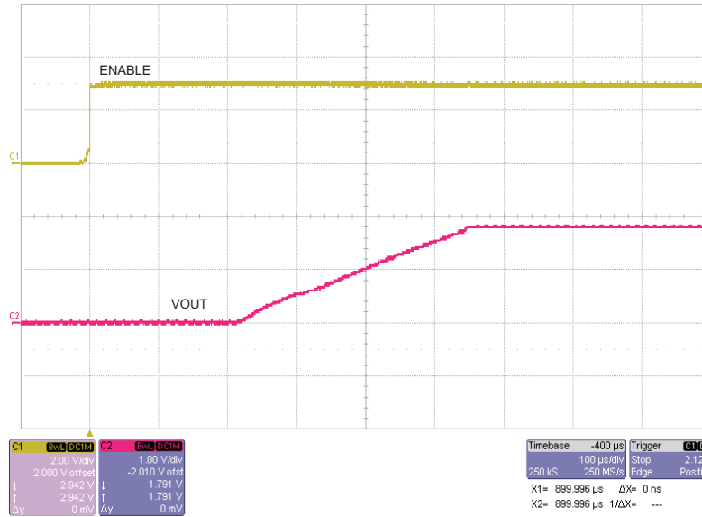
Figure 1. Start-up From Enable, V_{in}=3\text{ V} , V_{out}=1.8\text{ V} , I_{load}=600\text{ mA}
