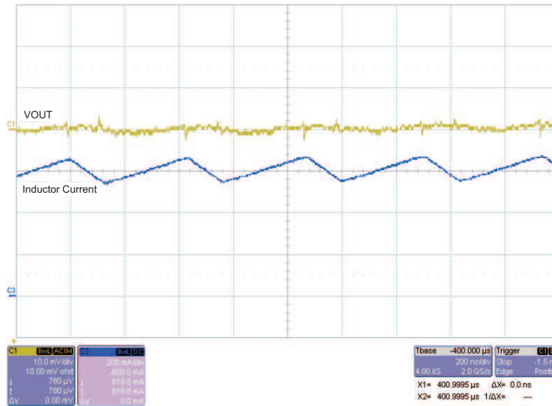
Figure 2. Output Voltage Ripple, V_{in}=3\text{ V} , V_{out}=1.8\text{ V} , I_{load}=600\text{ mA}
